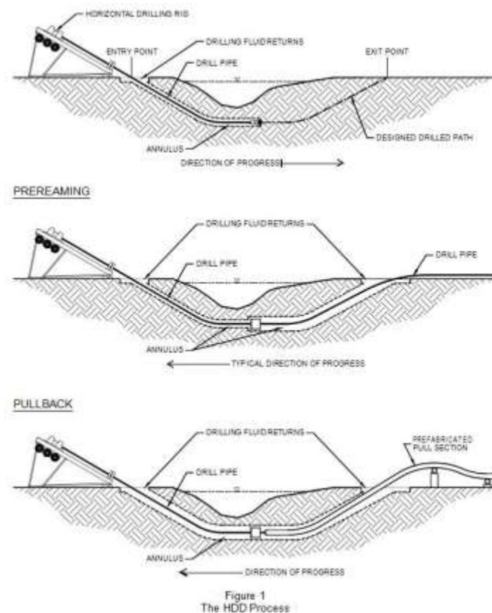
Figure 1.3: Cross-section of typical HDD construction method 4
